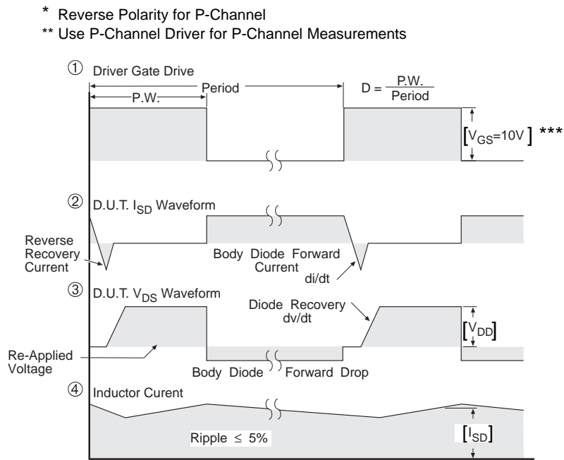
Fig 12. For P-Channel HEXFETS
